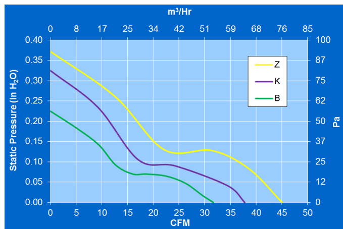
PERFORMANCE GRAPH
