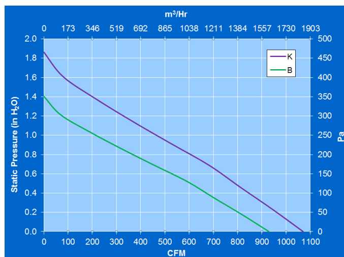
PERFORMANCE GRAPH
