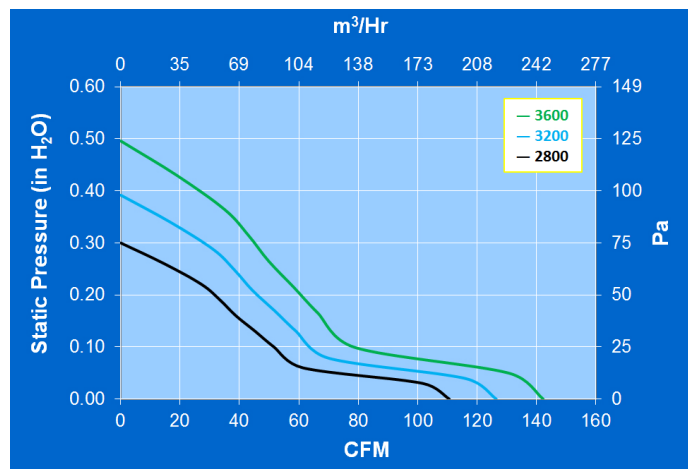
PERFORMANCE GRAPH
