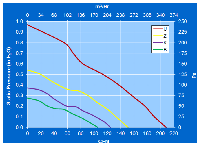
PERFORMANCE GRAPH
