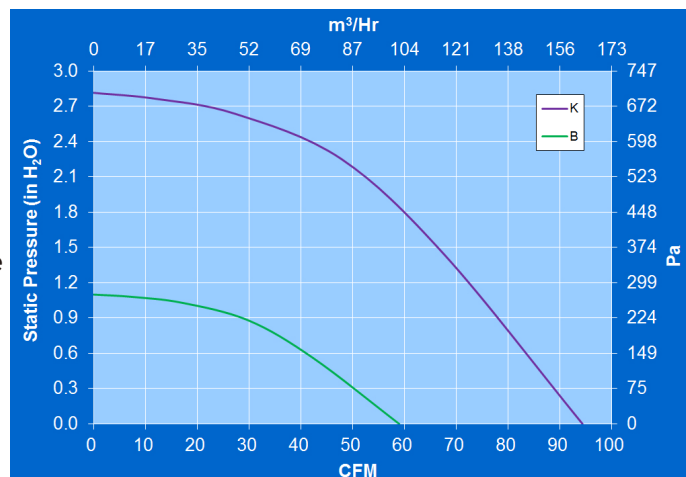
PERFORMANCE GRAPH
