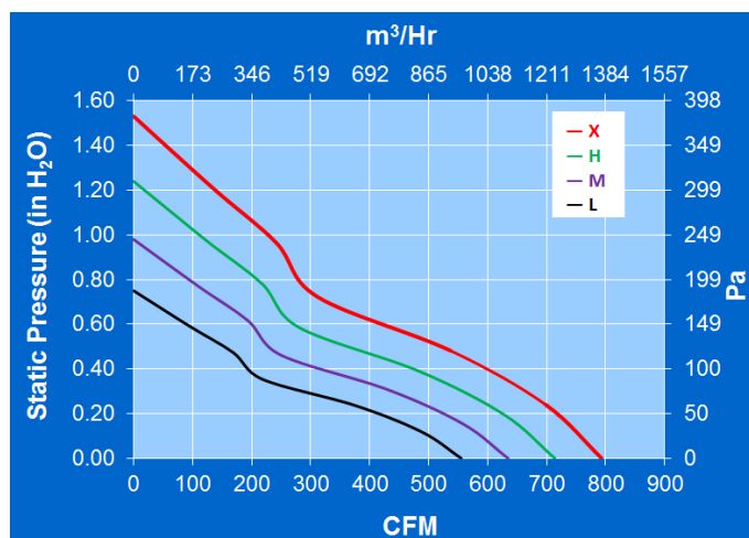
PERFORMANCE GRAPH
