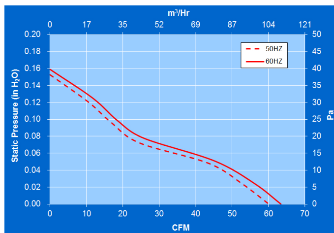
PERFORMANCE GRAPH
