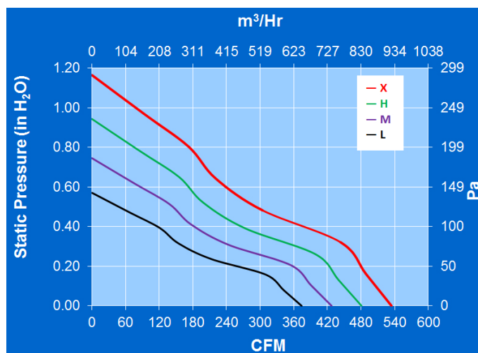
PERFORMANCE GRAPH
