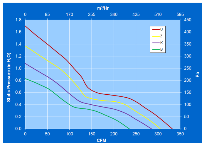
PERFORMANCE GRAPH
