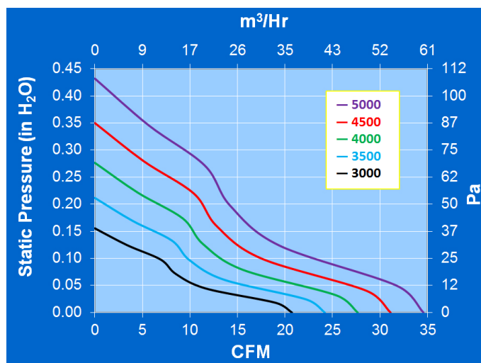
PERFORMANCE GRAPH
