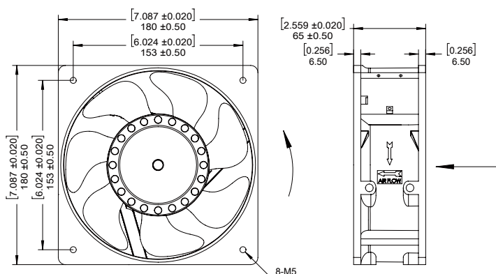
MECHANICAL DRAWING
